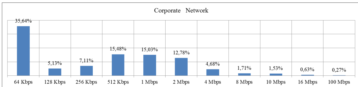
Figure 4 – Percentage of circuits by bandwidth
